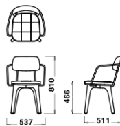
Arm Chair U W537xD511xH810/ SH466/7.5kg
