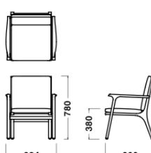
Lounge Chair W624xD600xH780/SH380/8.5kg
