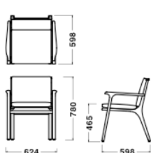
Dining Armchair W624xD598xH780/SH465/8.5kg
