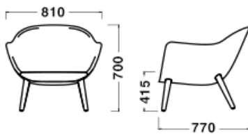
Chair 4-legs W810 × D770 × H700/ SH415/20.0kg
