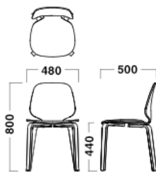
Chair W480xD500xH800/ SH440/6.2-6.3kg
