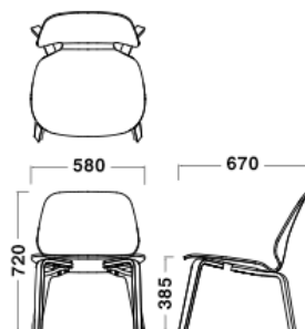
Lounge Chair W580xD670xH720/ SH385/7.9-9.8kg
