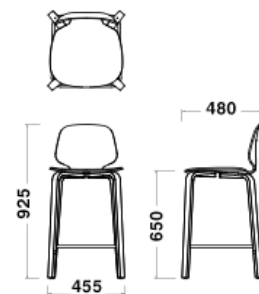
Stool W455xD480xH925/ SH650/6.2-6.3kg
