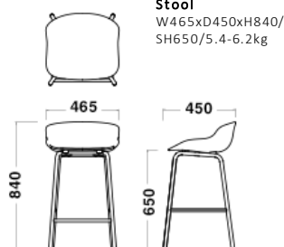
Swivel Chair W725xD725xH780-920/ SH380-520/10.2-11.5kg
