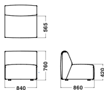
Sofa 1seater W840xD860xH760/SH420/29.8kg
