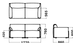
Sofa 2seater with arms W1770xD860xH760/SH420
