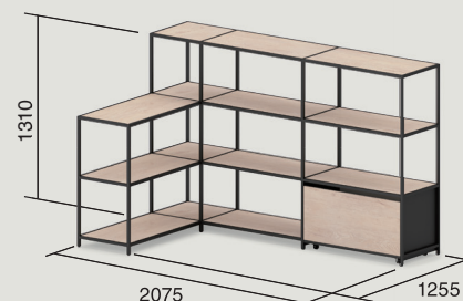
PLAN 02 L-shape
