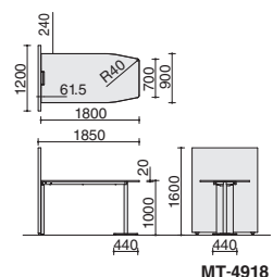
Counter table
