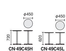
Disc base
